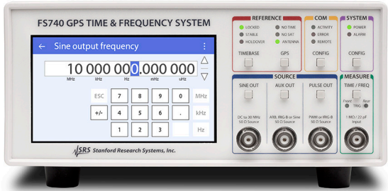
FS740 front panel
