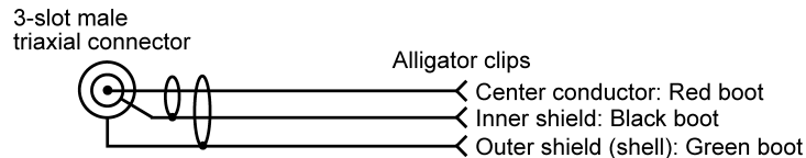
Figure 2: Model 237-ALG-2 schematic
